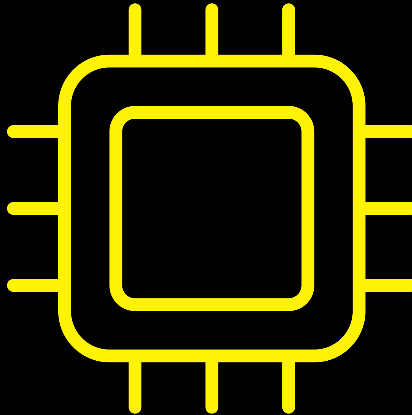
Service Worker
